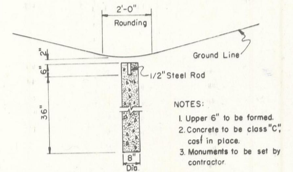
REFERENCE MONUMENT SECTION
