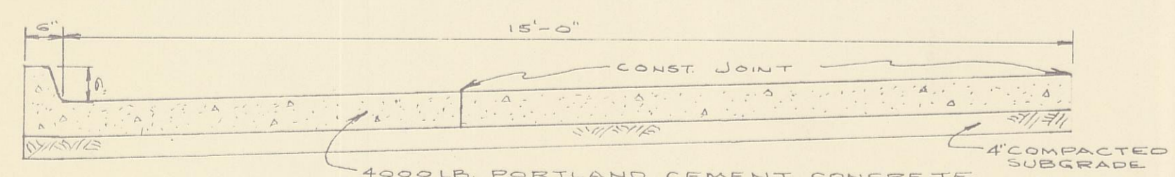
TYPICAL STREET HALF SECTION SCALE: 1/2" = 1'-0"
